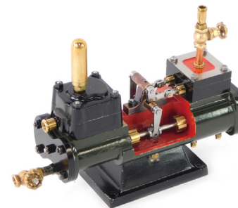
A scratch built steam boiler feed pump, possibly Stuart Turner, 15.5cm wide. SOLD for £400
